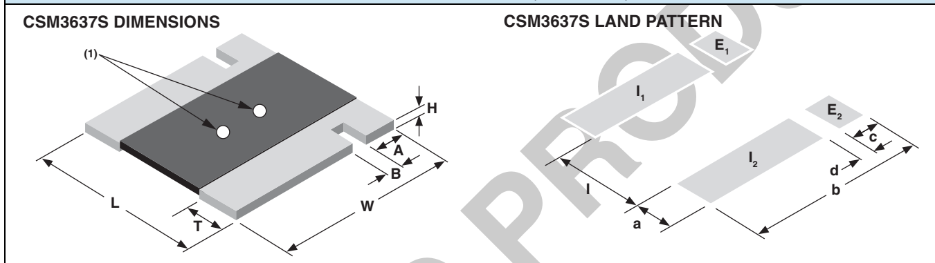
DIMENSIONS - TOLERANCES ± 0.010 (± 0.254)
